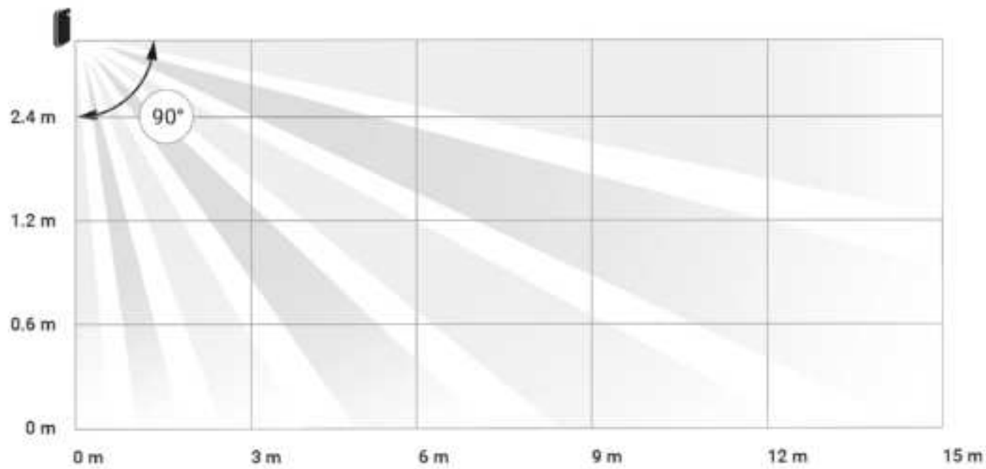
Horizontal and vertical detector's angles of view
