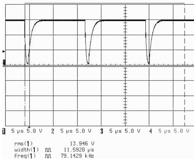
Figure 4.13 PFC Gate Switching at 4VDC
