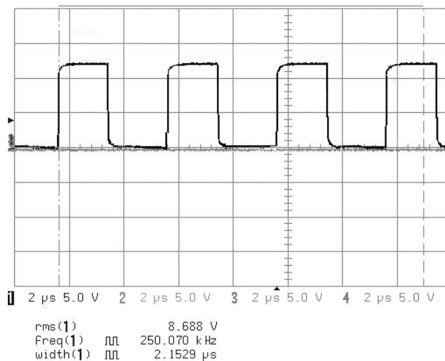
Figure 4.10 Gate Switching, View A
