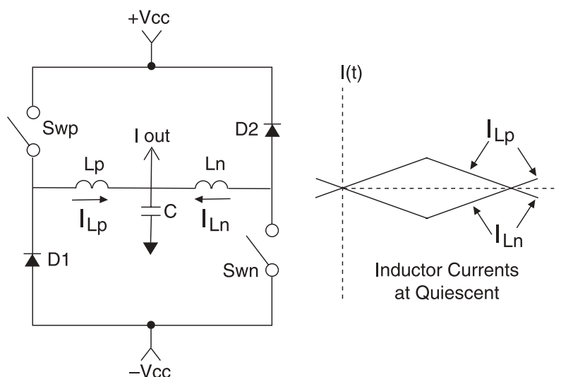
Figure 4.1 BCA Operation
