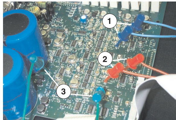
Figure 4.6 Shorting Jumpers
