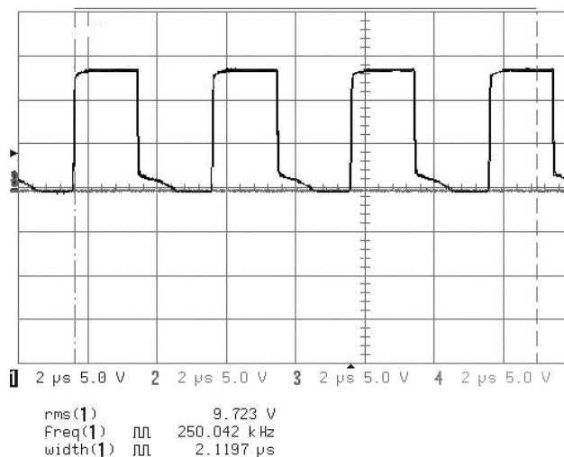
Figure 4.11 Gate Switching, View B
