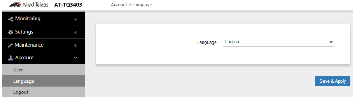
Figure 84. Language Window
