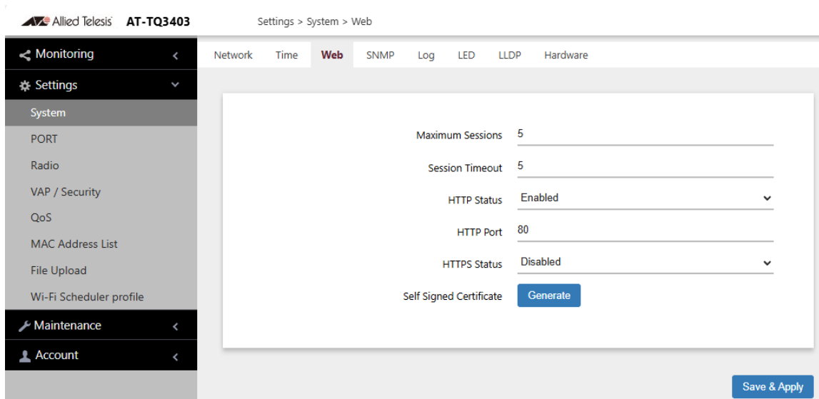
Figure 19. Web Window
