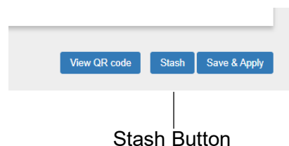
Figure 7. Stash Button
