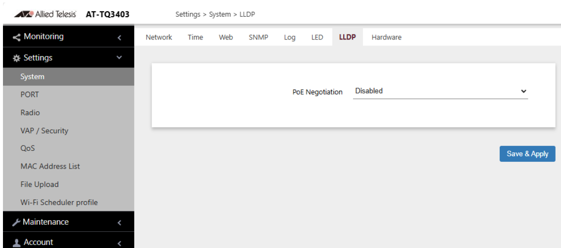
Figure 26. LLDP Window
