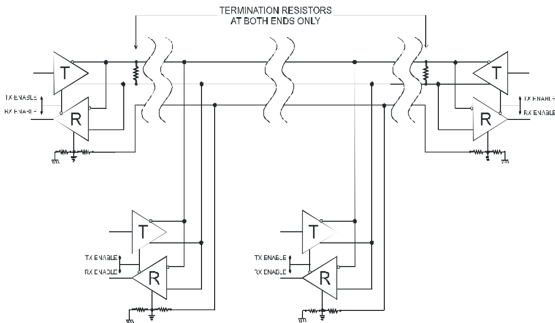
Figure A-1: Typical RS485 Two-Wire Multidrop Network
