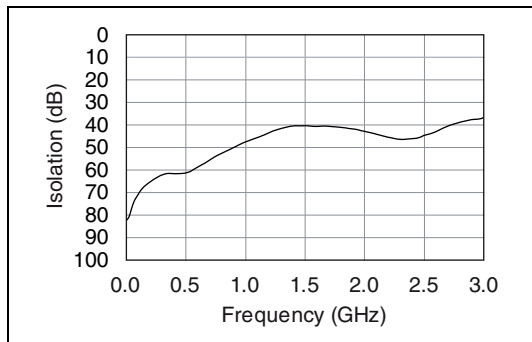
Figure 3. Typical Isolation
