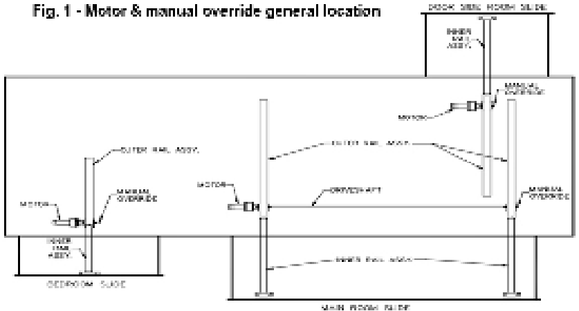
Fig. 1 - Motor & manual override general location
