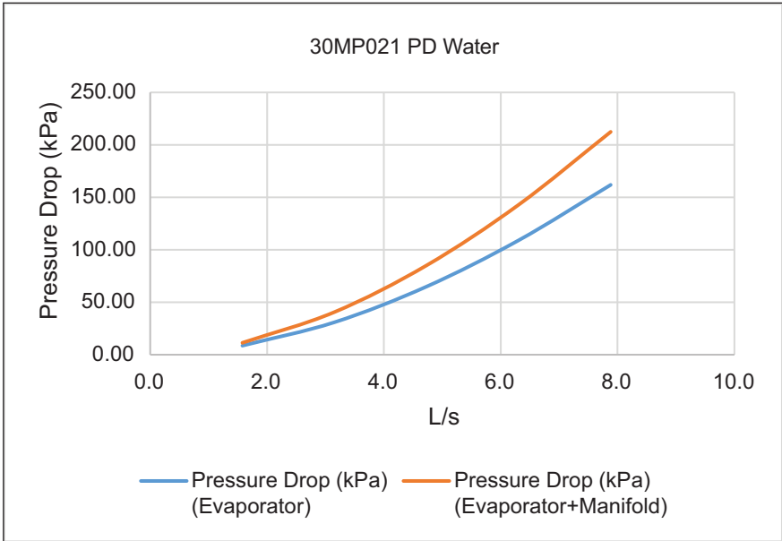
Condenser Water Pressure Drop Curve — SI
