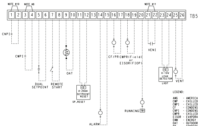
TYPICAL MAIN POWER & CONTROL CONNECTIONS
