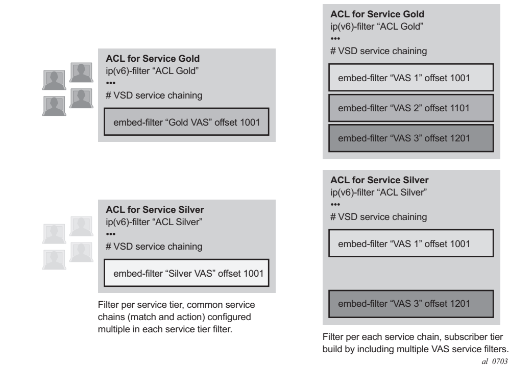
Figure 31 ACL filter modeling for ESM Service Chaining
