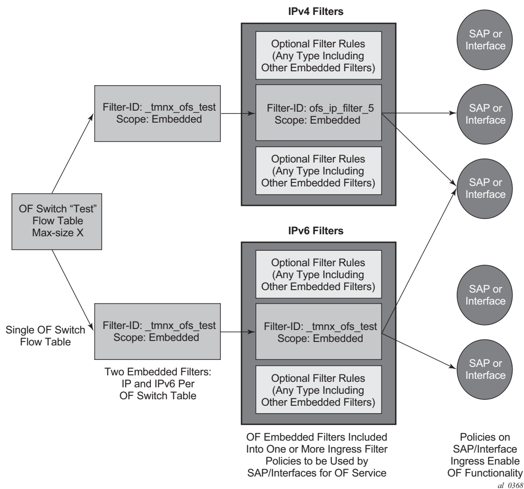
Figure 36 OF Flow Table Mapping to Router/Switch Service Infrastructure Example — switch-defined-cookie Disabled
