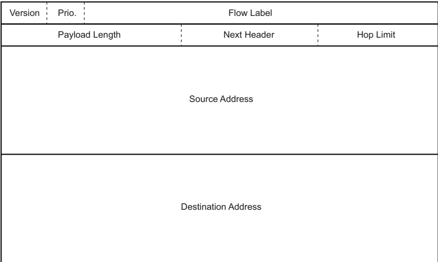
Figure 3 IPv6 Header Format
