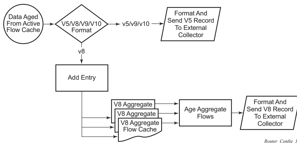
Figure 39 V5, V8, V9, V10, and Flow Processing
