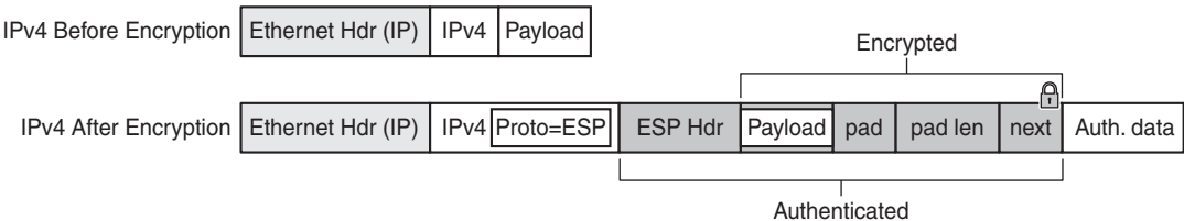
Figure 15 Router Interface Encryption Packet Format (IPsec Transport Mode)
