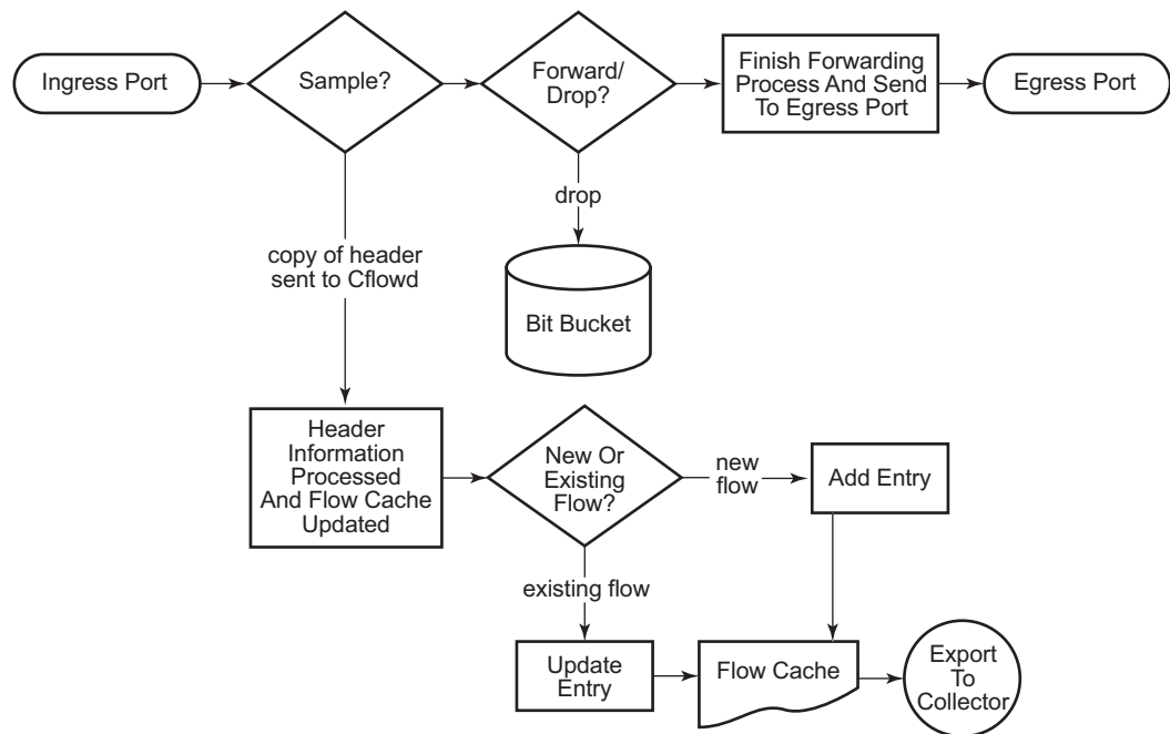
Figure 38 Basic Cflowd Steps
