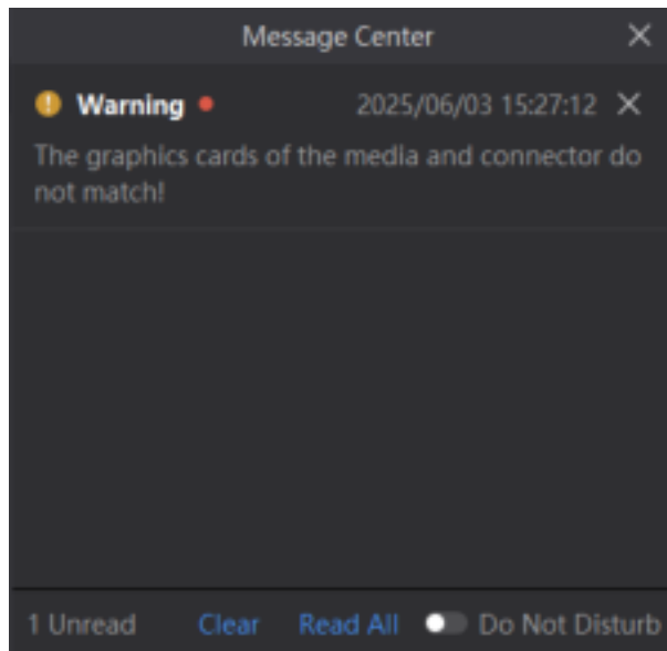
Figure 3-5 Message center
