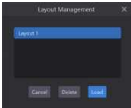
Figure 3-3 Load layout
