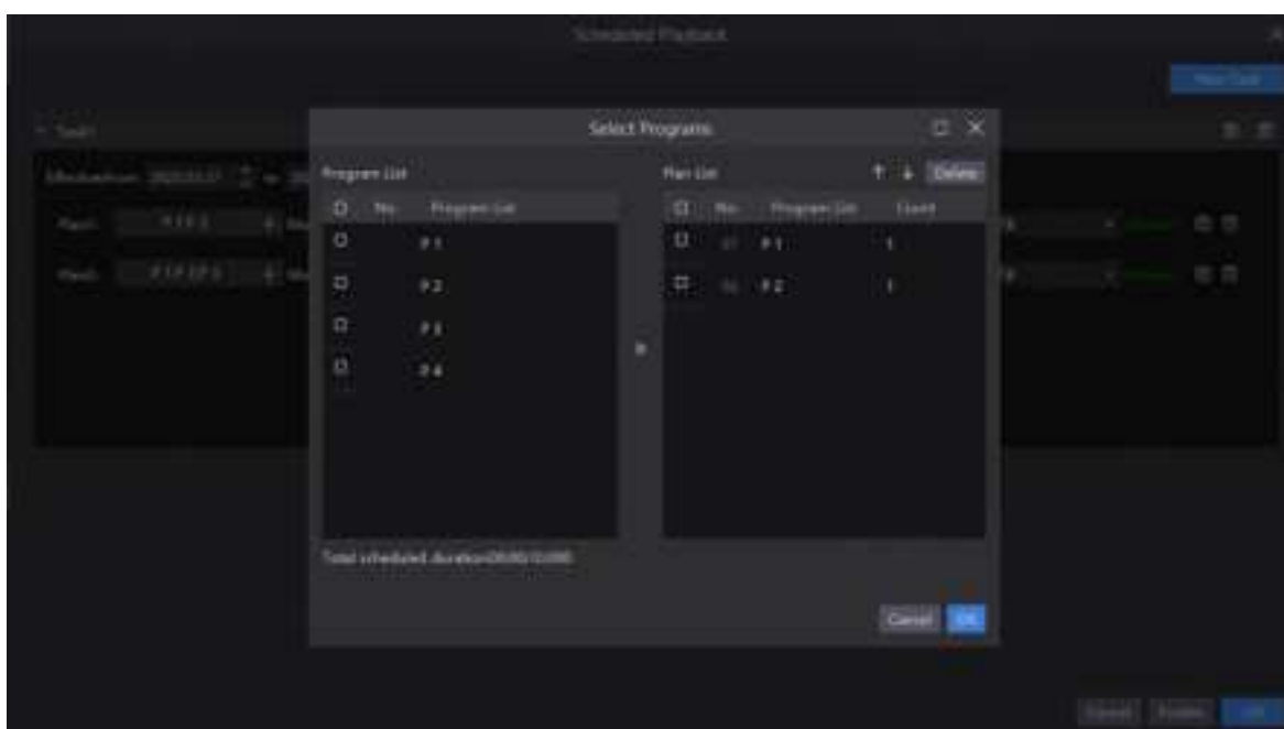
Figure 4-59 Select programs
