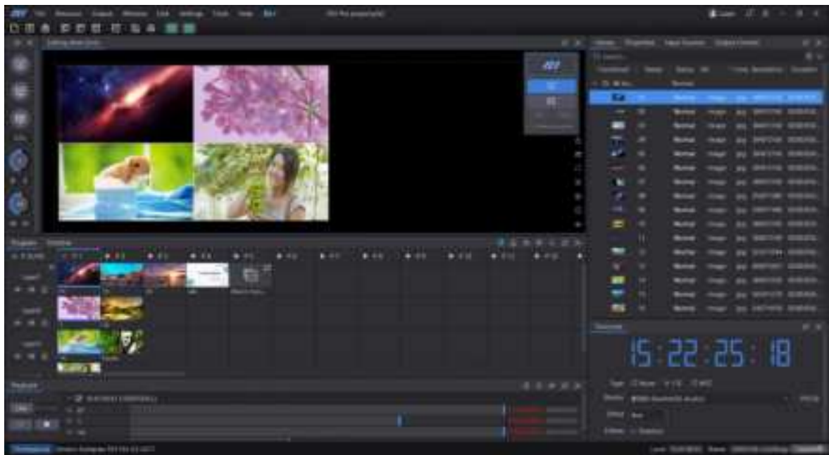
Figure 3-1 User interface
