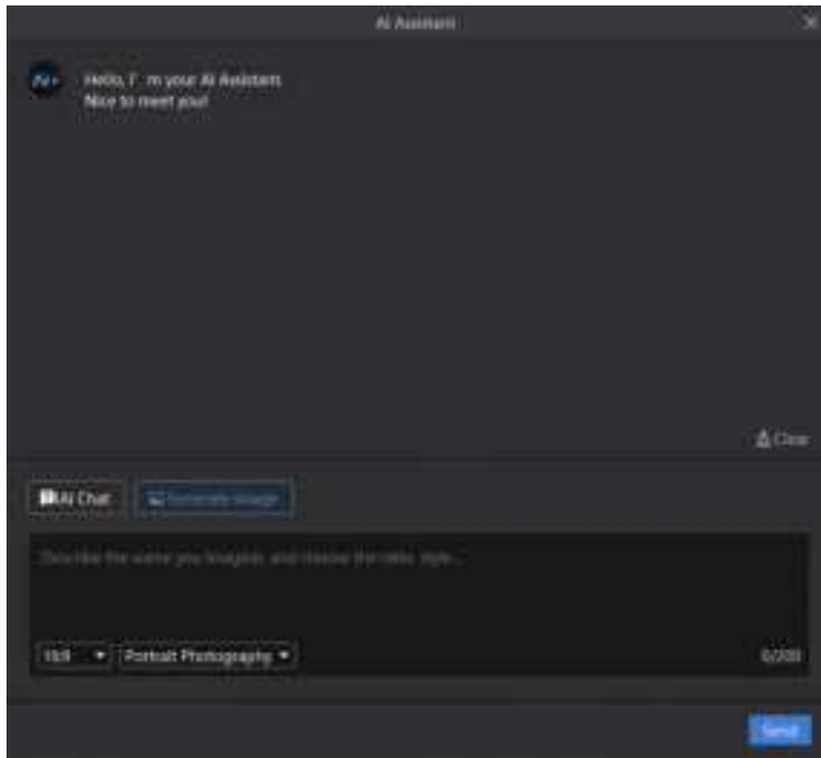
Figure 9-6 Image generation
