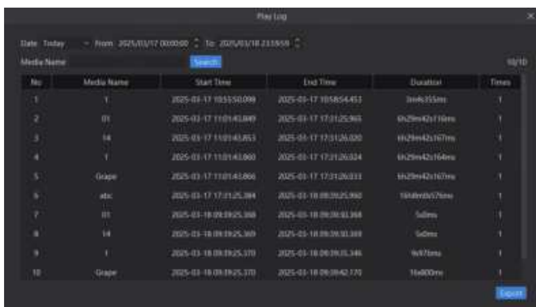
Figure 7-3 Play log - 2
