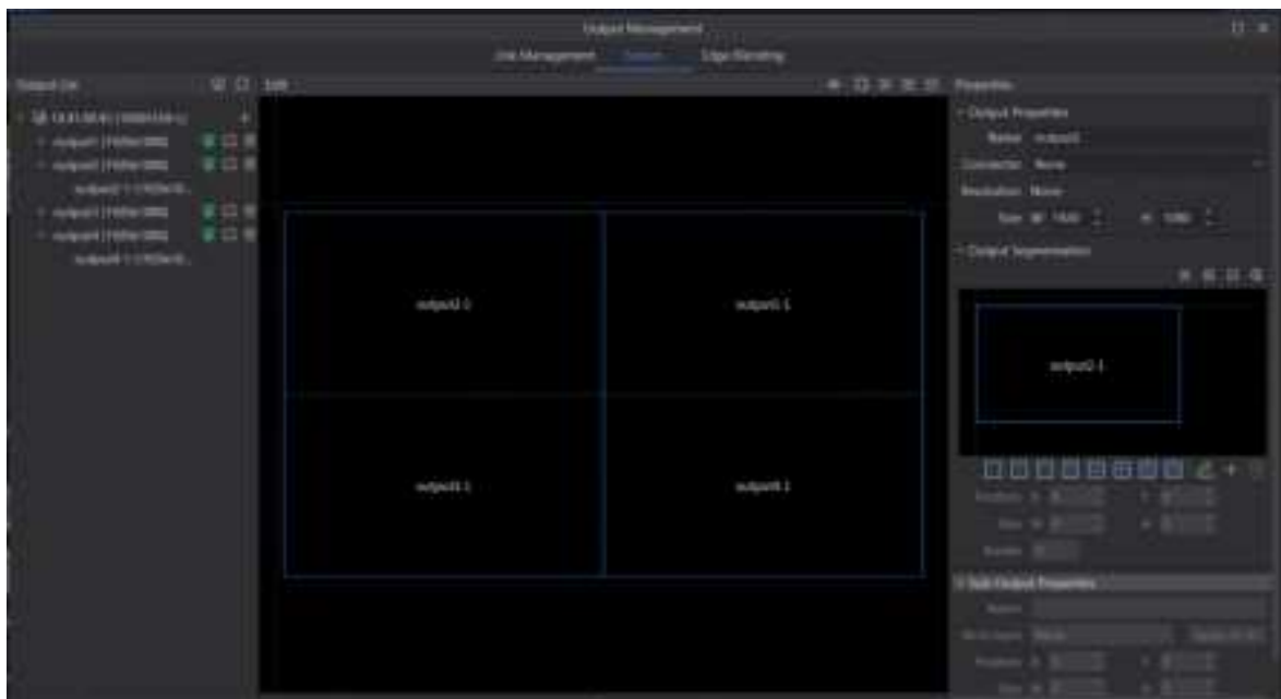
Figure 4-11 Screen management
