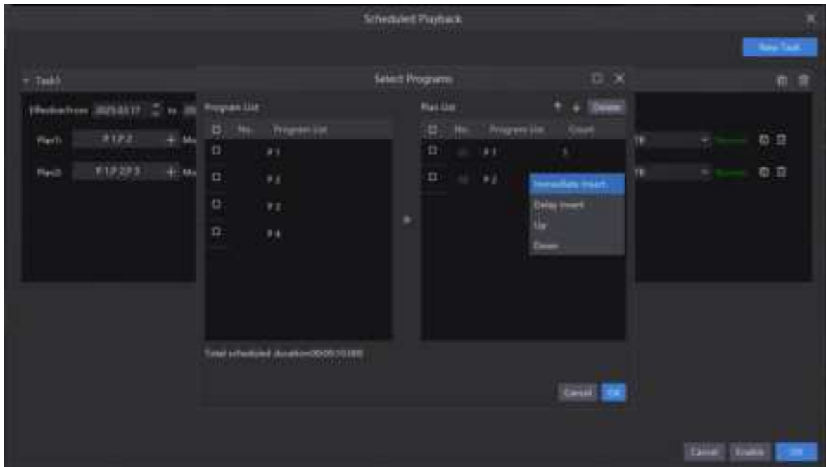
Figure 4-60 Insert programs
