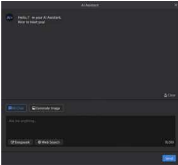
Figure 9-5 AI assistant
