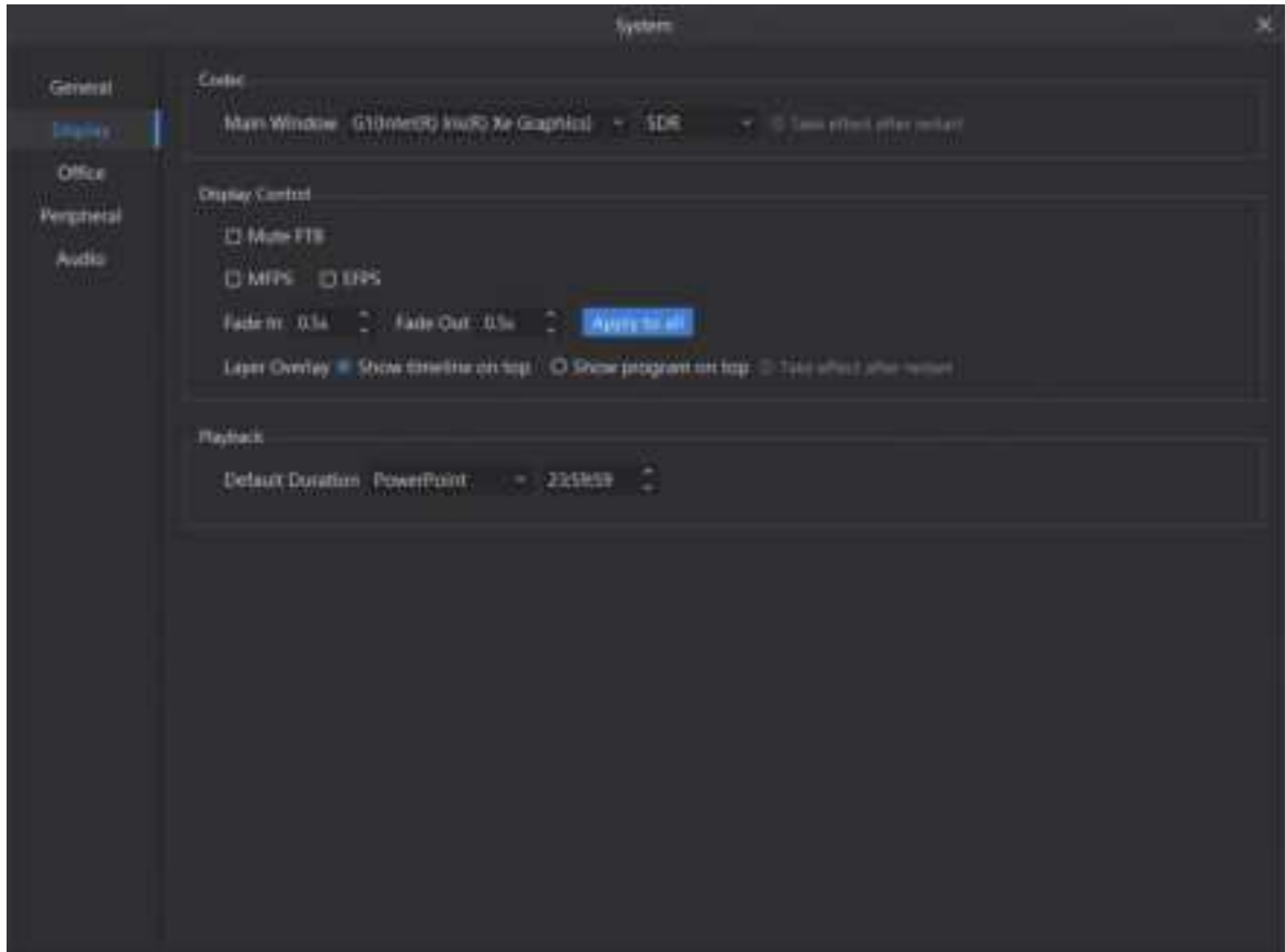
Figure 6-2 Display settings
