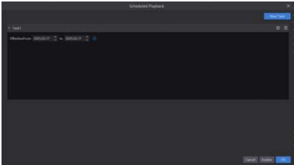
Figure 4-55 Playback tasks
