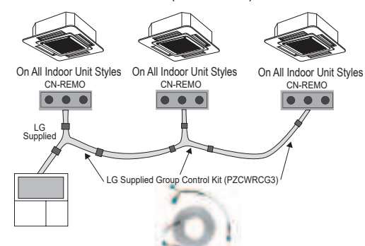
Figure 43: Example of Indoor Unit Group to Zone Controller Connections (CN-REMO).
