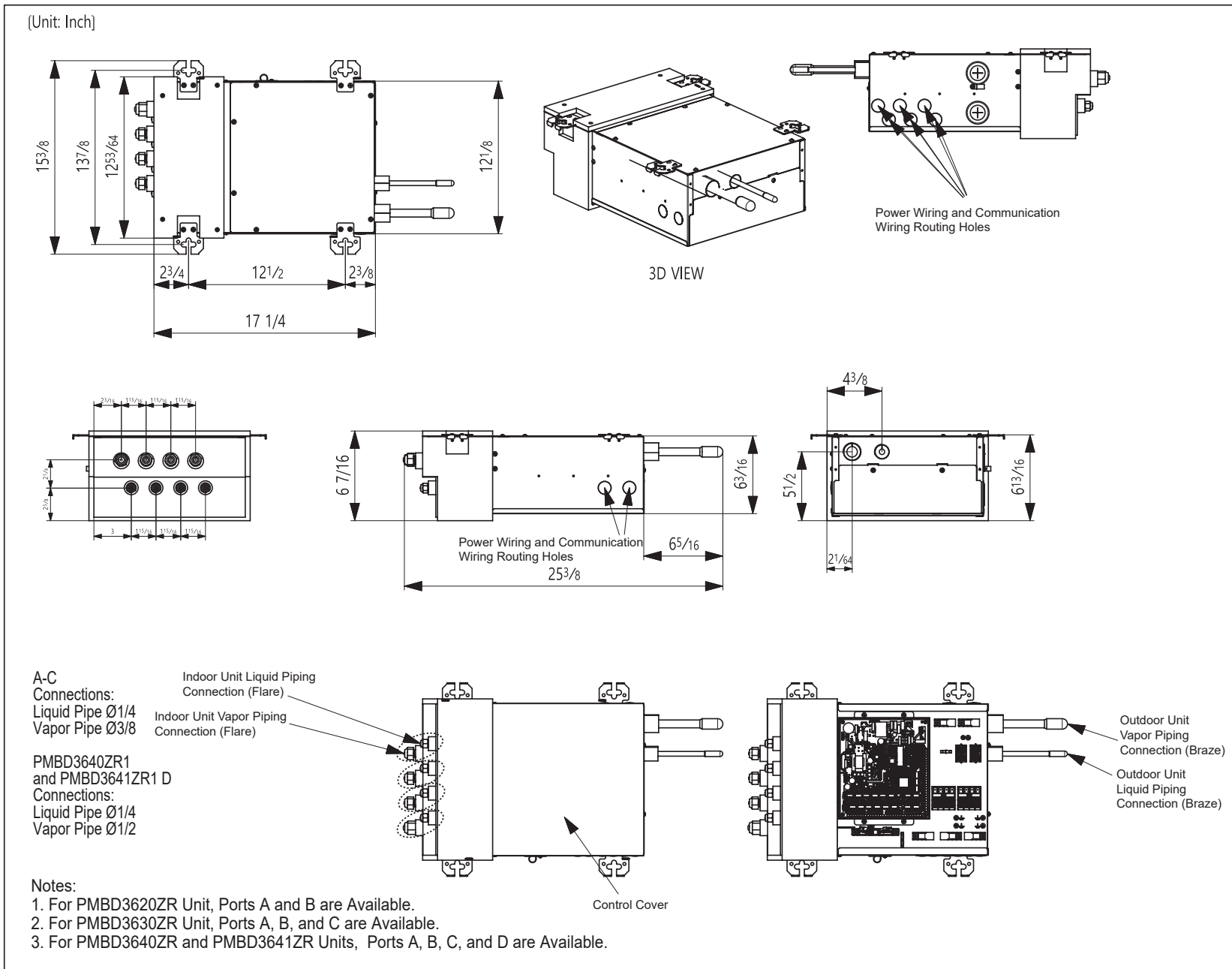
Figure 24: PMBD3620ZR, PMBD3630ZR, PMBD3640ZR, and PMBD3641ZR Dimensions.
