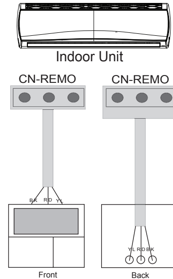
Figure 41: Another Example of Indoor Unit to Zone Controller Connection.
