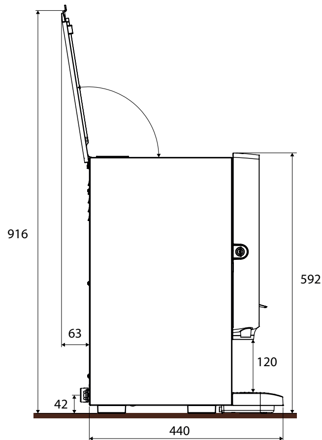
Side view with opened top cover (+80 mm space at the rear side)
