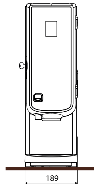
Front side (100 mm at both sides of the machine for service/maintenance and ventilation)
