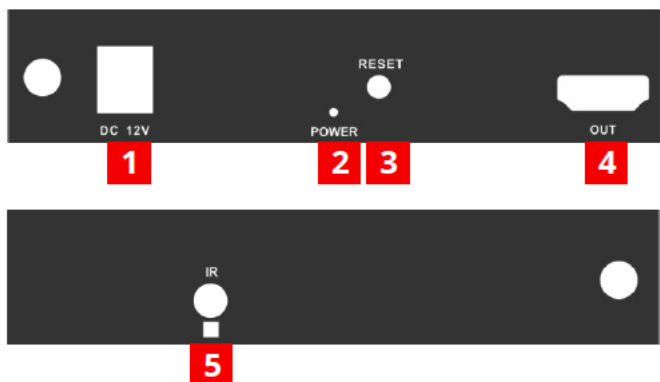
Figure 2: Receiver (RX)
