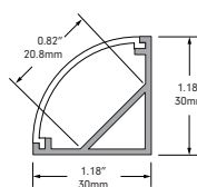
FRE-CHAN-SLV-6.5 Anodized Aluminum Extrusion, available in 6.5' lengths
