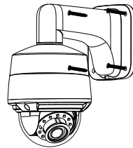
Figure 3-2 Wall installation
