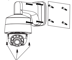
Figure 3-10 Installing on bracket
