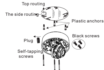
Figure 3-4 Installing housing
