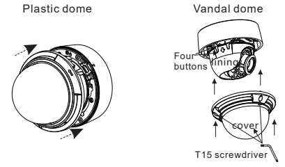
Figure 3-8 Assembling lining and base
