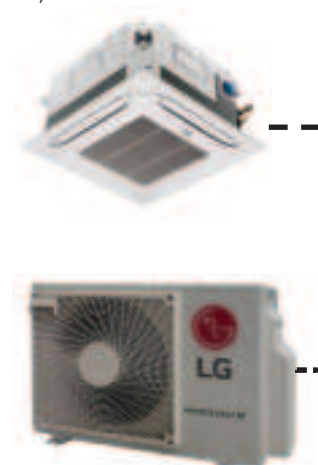
Figure 3: Four-Way Ceiling Cassette System (LC098HV4 and LC128HV4 Models).
