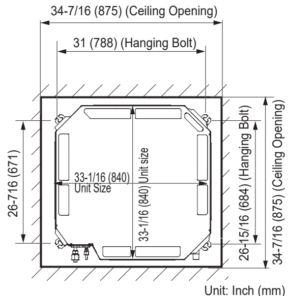
Figure 44: 3 x 3 Cassette Ceiling Opening Dimensions and Bolt Locations.
