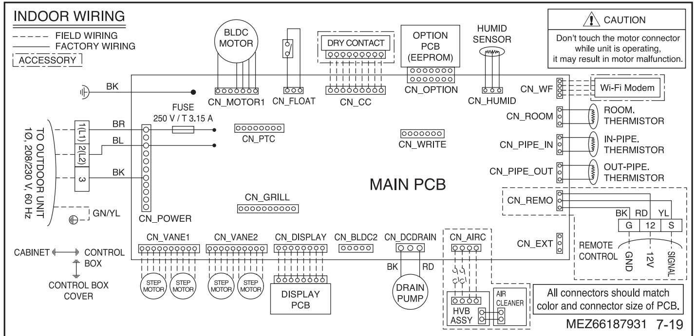
Figure 26: LCN248HV, LCN368HV, and LCN428HV Four-Way Ceiling Cassette Indoor Unit Wiring Diagram.
