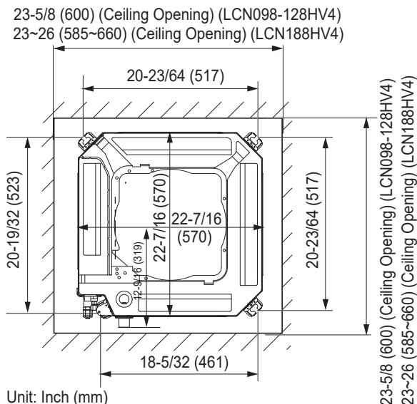
Figure 43: 2 x 2 Cassette Ceiling Opening Dimensions and Bolt Locations.
