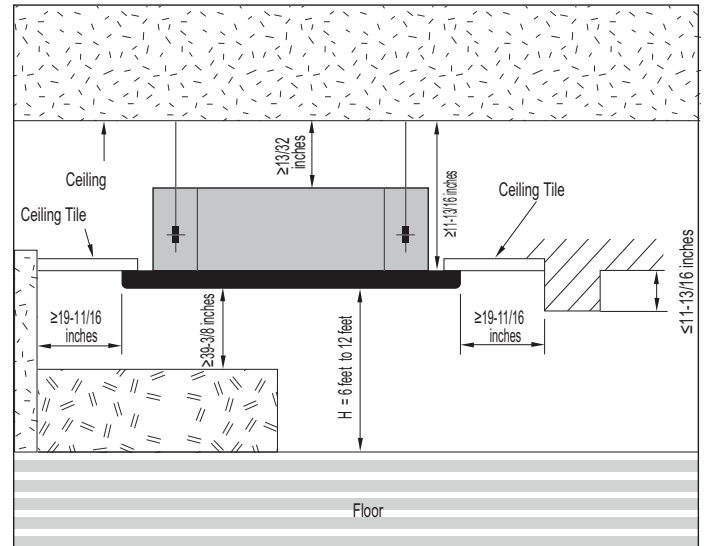
Figure 42: Indoor Unit Clearance Requirements.
