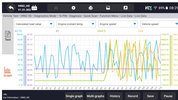
Figure 9-23 Sample Merge Graph Screen
