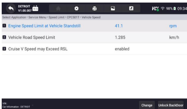
Figure 12-3 Sample Test Result Screen
