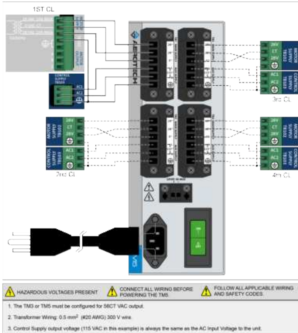
Figure B-3: System Interconnect Example (CL)
