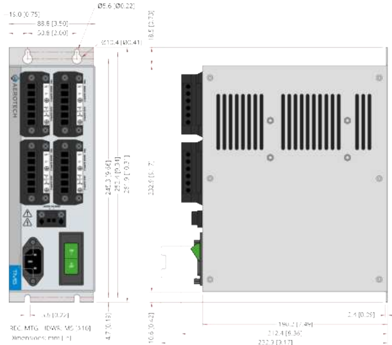
Figure 1-2: Dimensions
