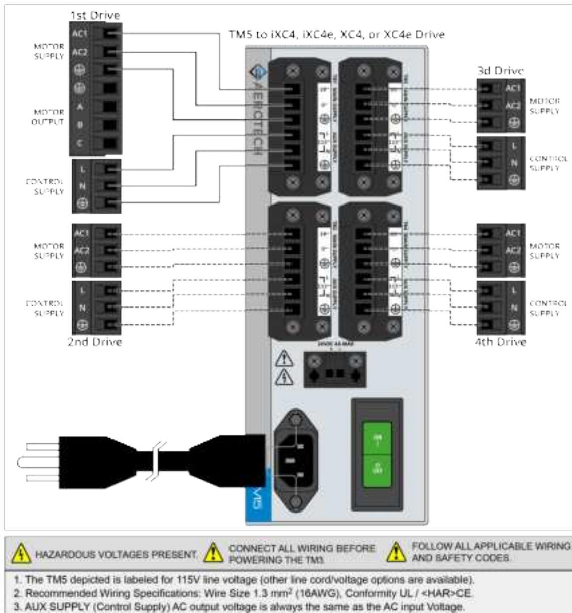
Figure 1-3: System Interconnect Example (iXC4/XC4 and iXC4e/XC4e)
