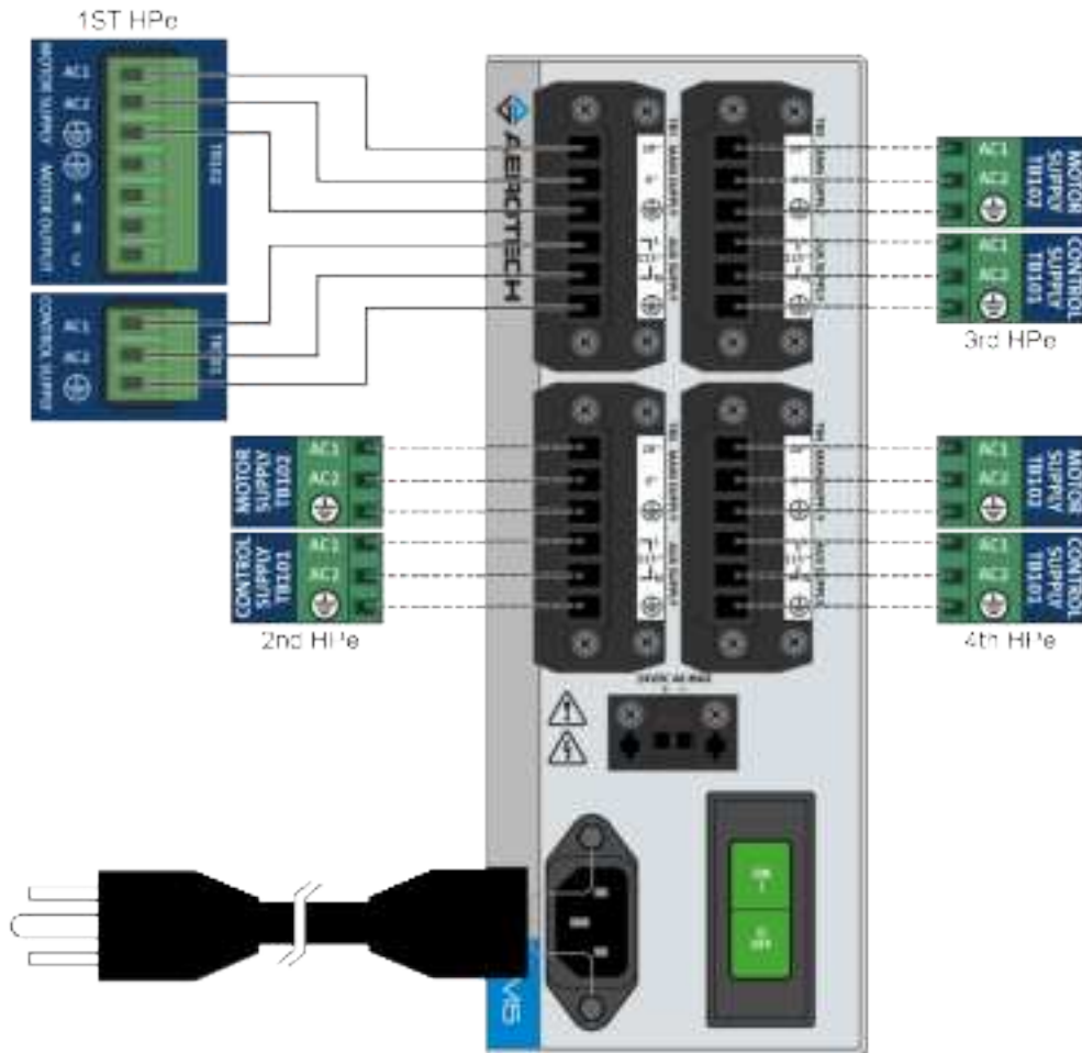
Figure B-1: System Interconnect Example (HPe)
