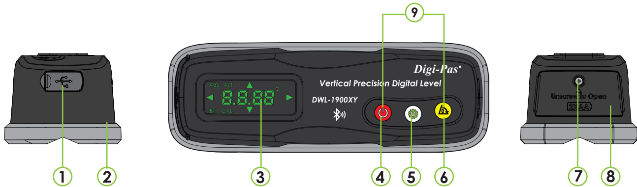
Figure 2. Overview of the Machinist Level
