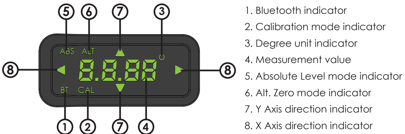
Figure 3. Machinist level display overview
