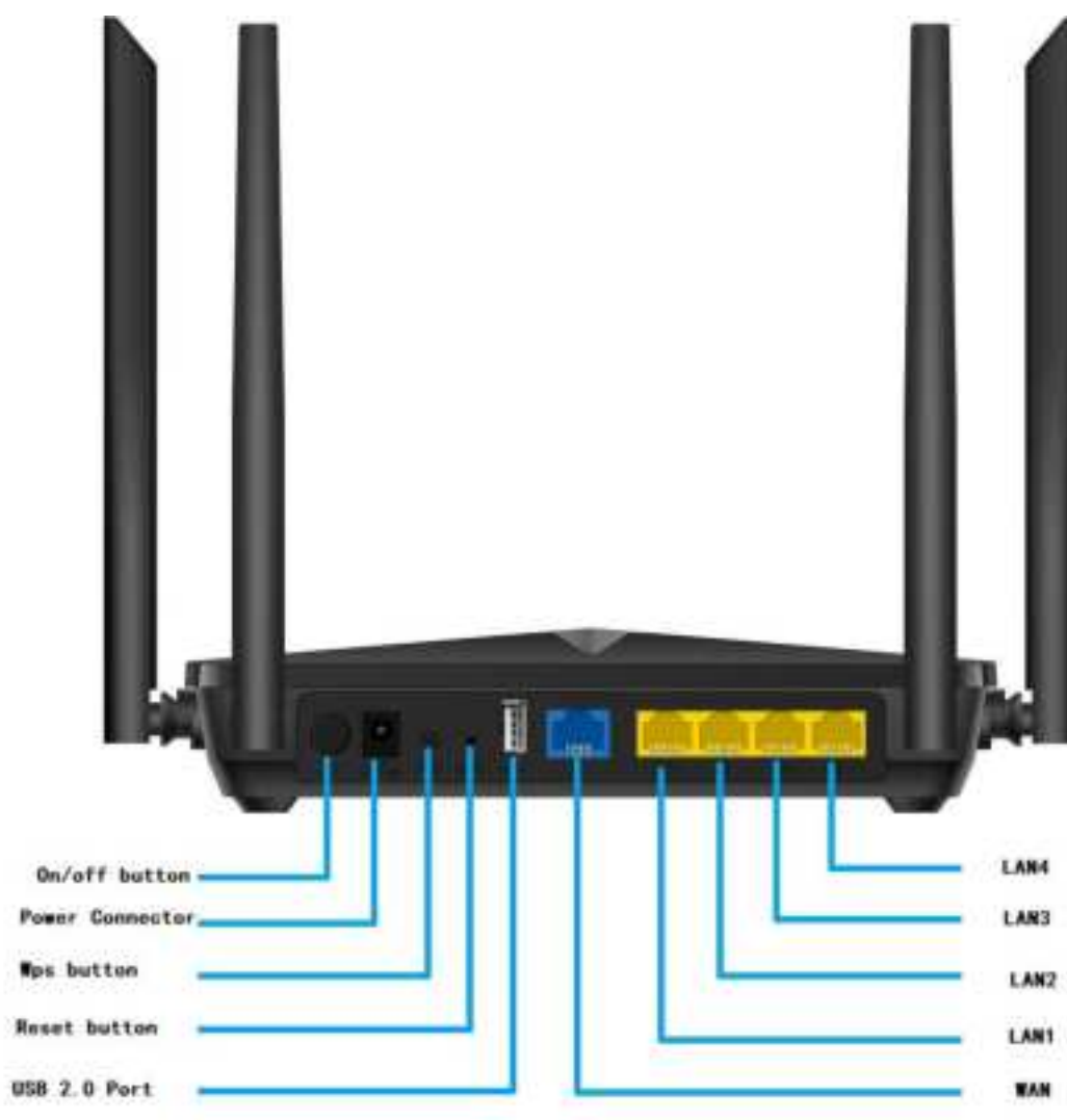
Figure 2-1-3-1 Rear Panel of the DIR-825M
