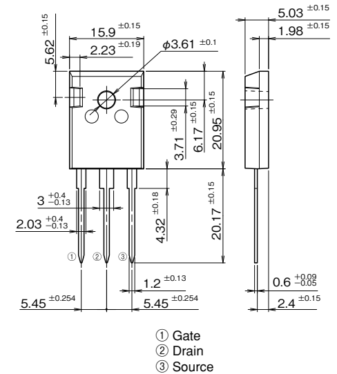
TO-247-P2
