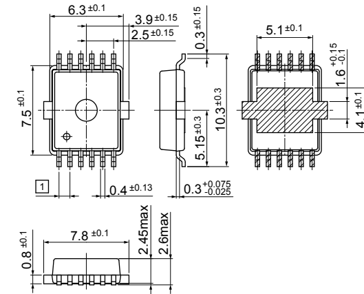
PSOP-12
