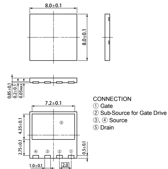
DFN8x8
