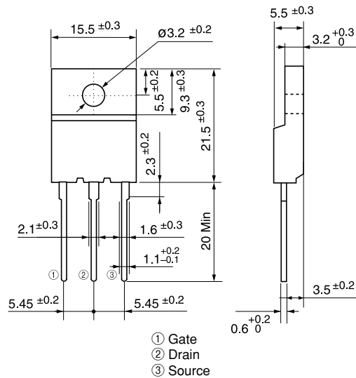
TO-3PF
