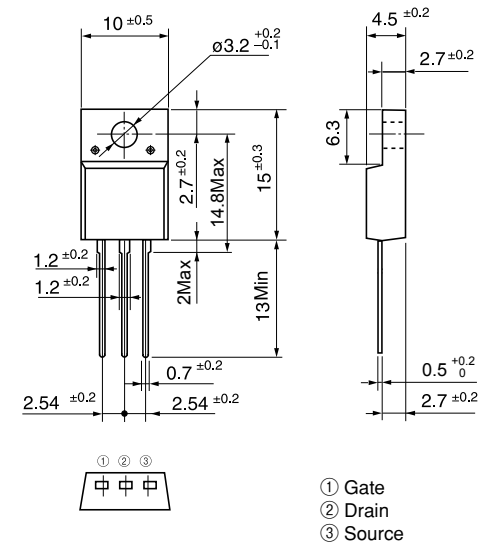
TO-220F(SLS)
