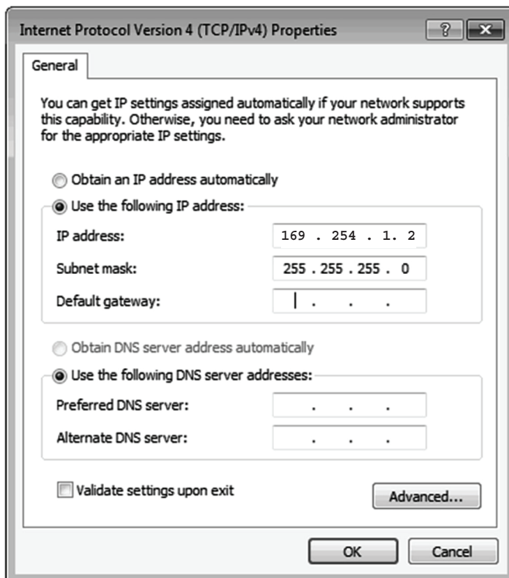
FIGURE 4-1. TCP/IPV4 WINDOW
