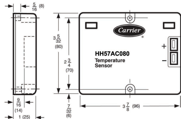
Fig. 4 — Temperature Sensor Specifications
