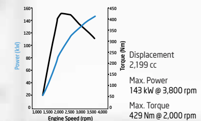
2.2L CRDi engine
