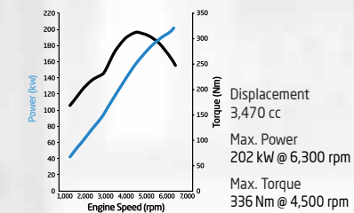
3.5L V6 engine
