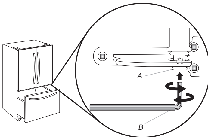
A. Bottom hinge pin B. 1/8" Hex-key wrench
