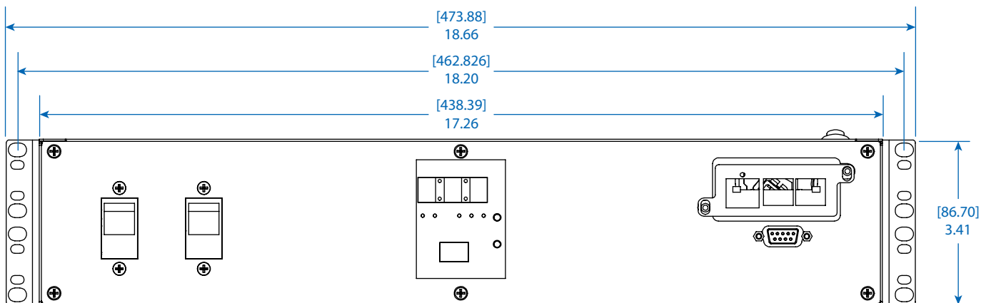
REAR VIEW
