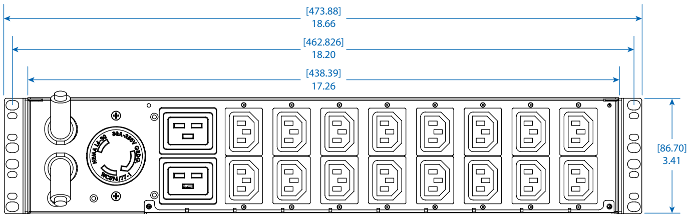
FRONT VIEW
