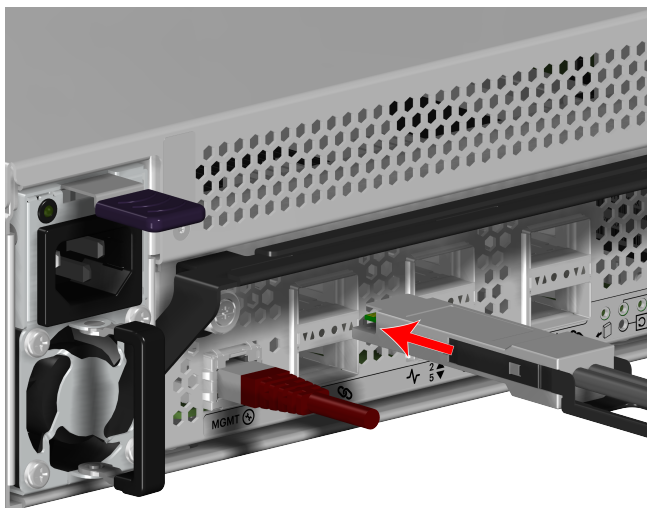
Figure 17: Connect QSFP28 Cable
