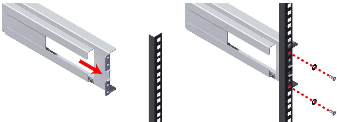
Figure 11: Install Front Rack Mount
