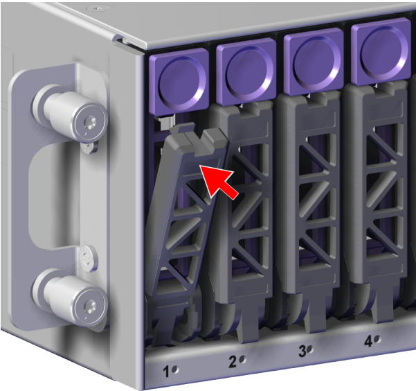
Figure 22: Drive Assembly Installation
