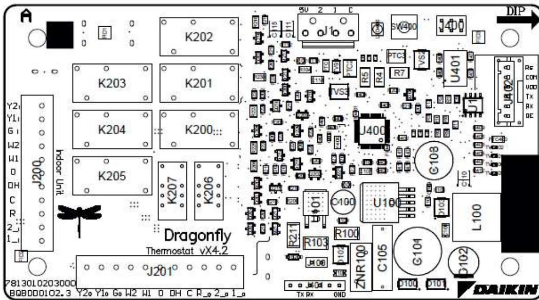
Images of PCB layout showing connector labeling below
