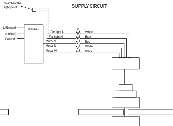
SUPPLY CIRCUIT
