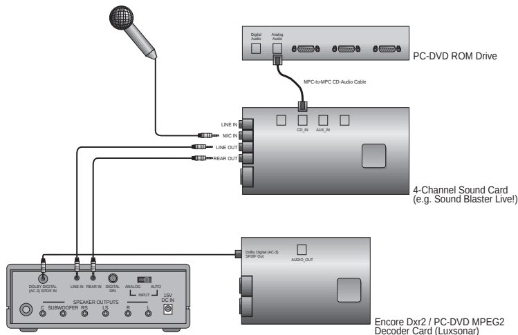
Connection Guide for DeskTop Theatre 5.1 DTT2500 Digital with Sound Blaster Live! and Creative PC-DVD system.
