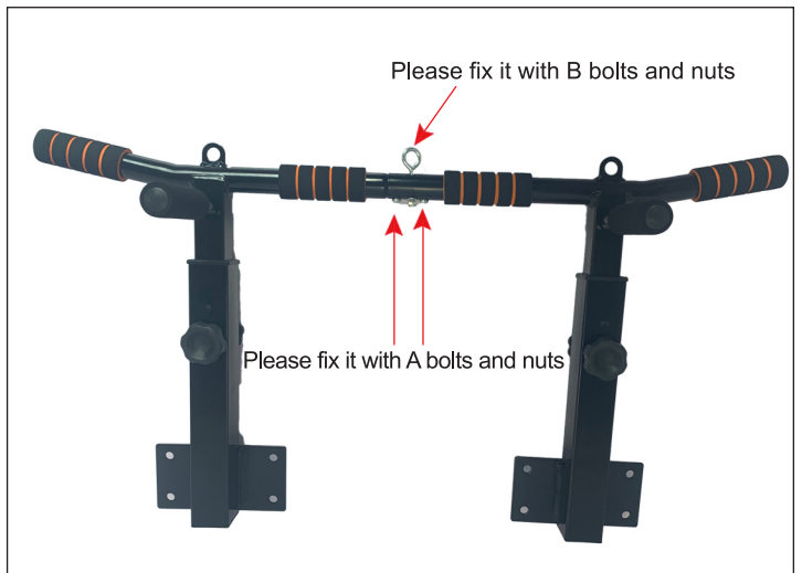
Step 4: Connect the left and right cross bar with A and B bolts and nuts, and tighten the bolts. And now it's completely assemble.
