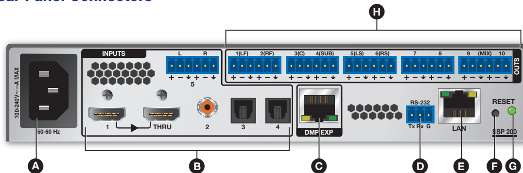
Figure 1. Rear Panel Connectors
