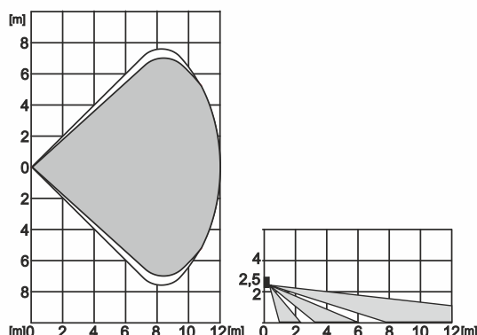
Figure 2: Coverage characteristics
