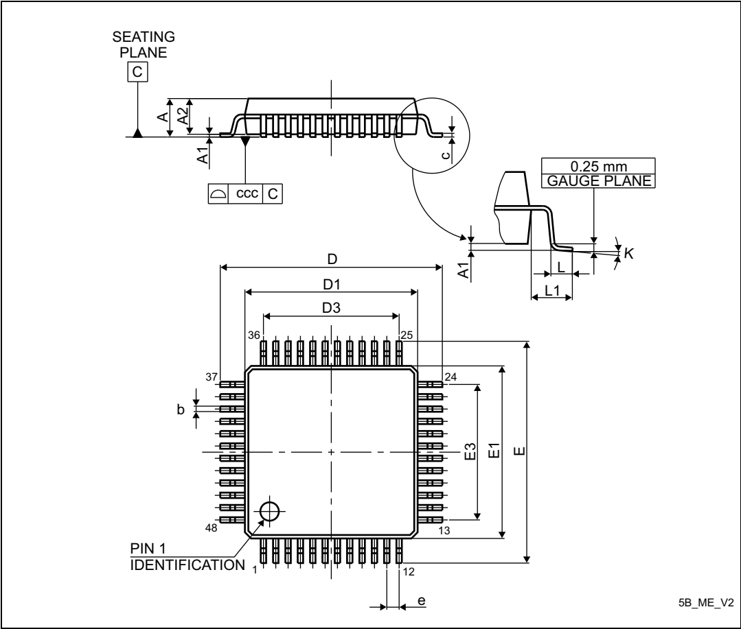
Figure 82. LQFP48 - Outline
