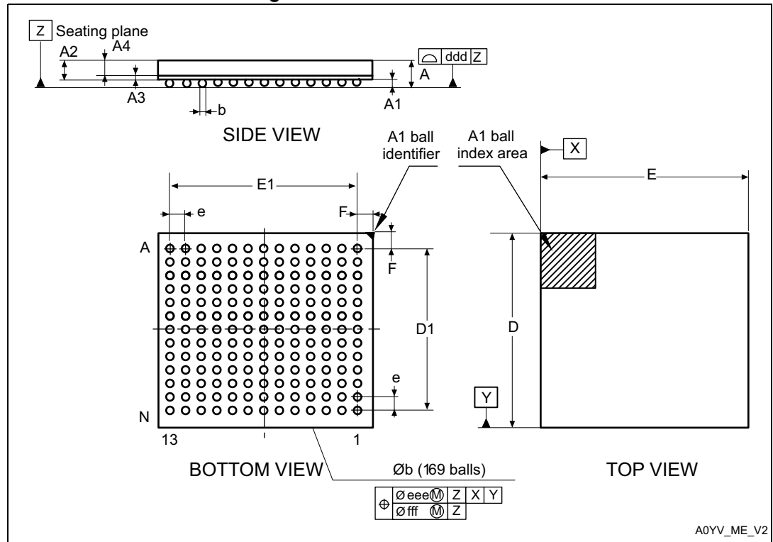
Figure 99. UFBGA169 - Outline
