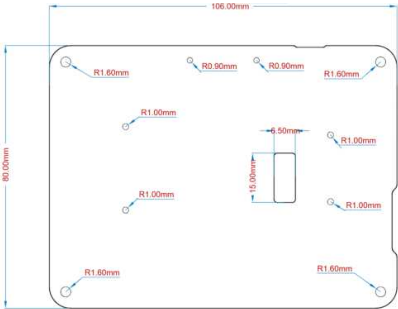
Mechanical View of Arduino GIGA Display Shield
