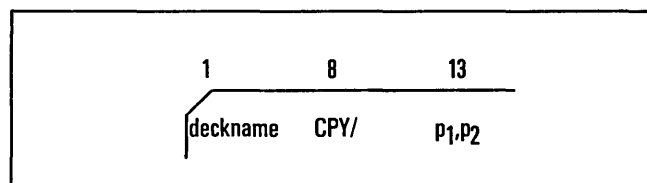
Figure 8-12. Second CPY/ Card Format
