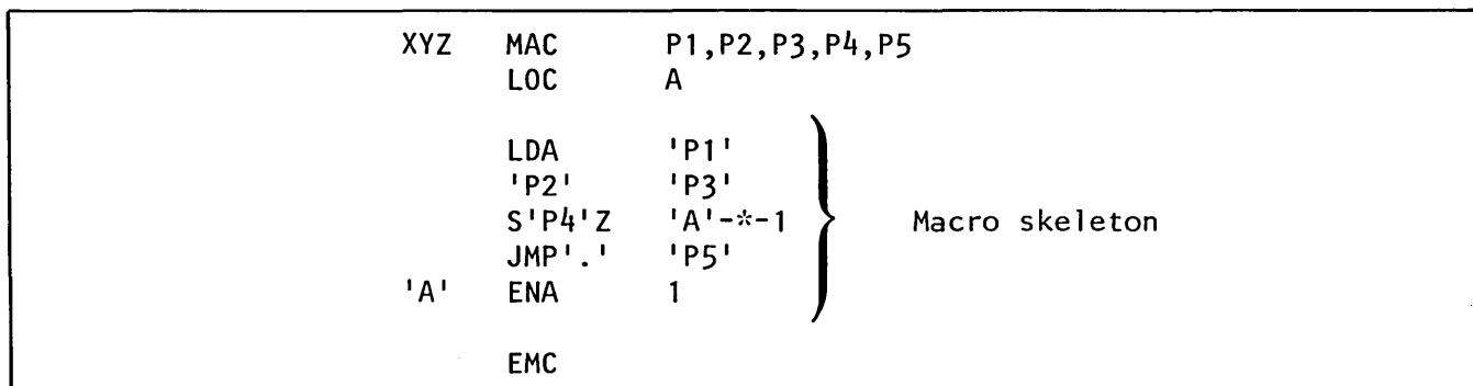
Figure G-26. Macro Skeleton
