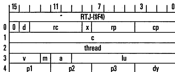
Figure 3-5. MOTION Request Calling Sequence
