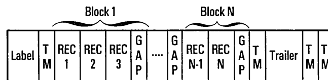
Figure F-3. Fixed-Length, Blocked Records
