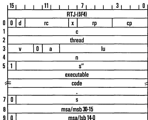
Figure 4-5. First Data Transfer Request Format
