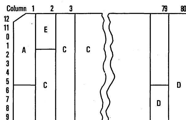
Figure 4-4. Subsequent Binary Format Cards
