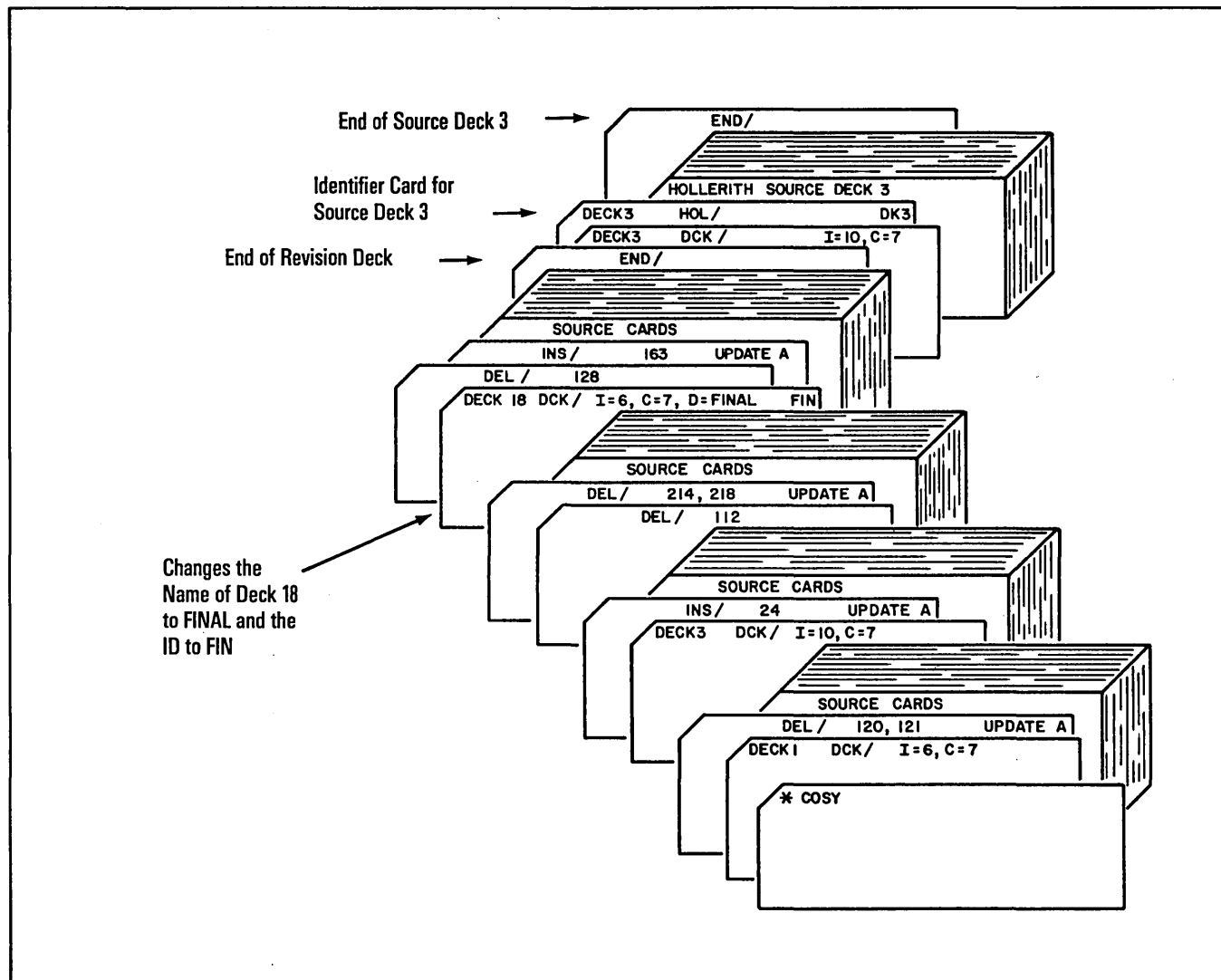
Figure 8-17. COSY Deck Updating
