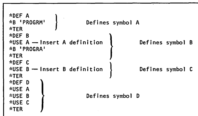
Figure 8-25. Six-Level Nesting of *USE Record
