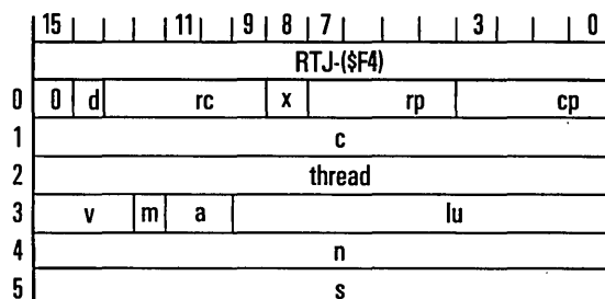
Figure 3-1. Macro-Generated Calling Sequence
