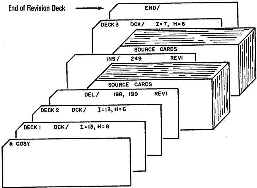
Figure 8-24. COSY Deck Conversion to Hollerith Library
