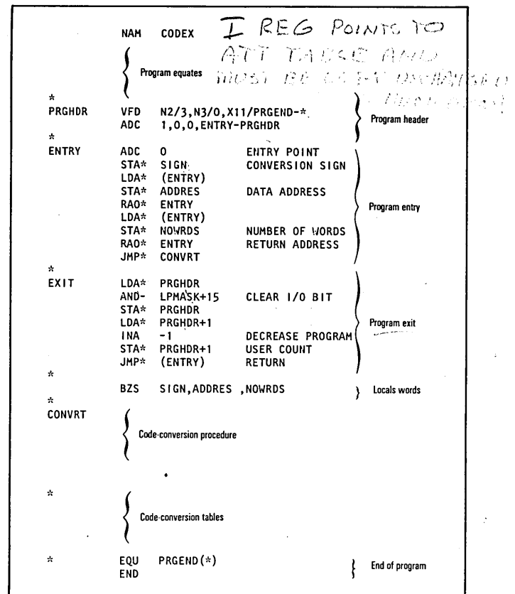
Figure B-10. Code-Conversion Structure
