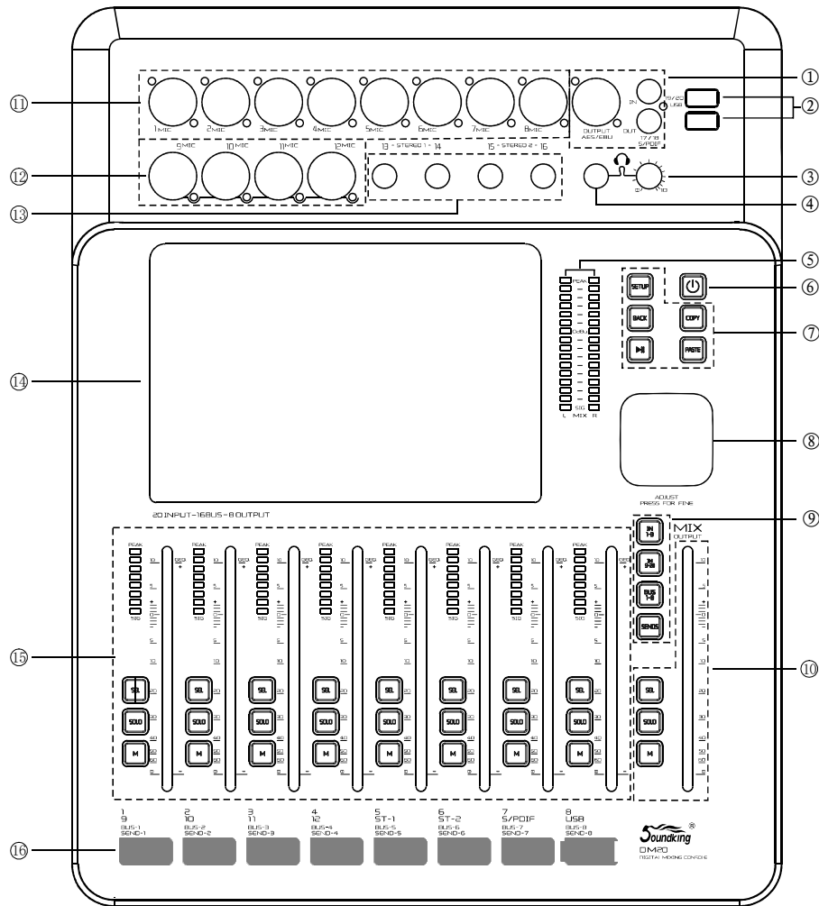
(DM20 Mixer panel)
