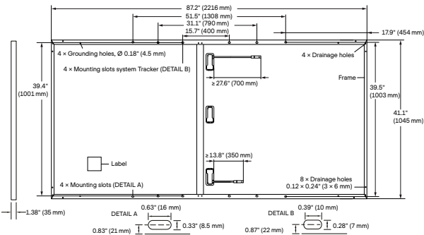
Fig. 1: External dimensions (in inch (mm)) and components for Q.PEAK DUO XL-G10.2 and Q.PEAK DUO XL-G10.c
