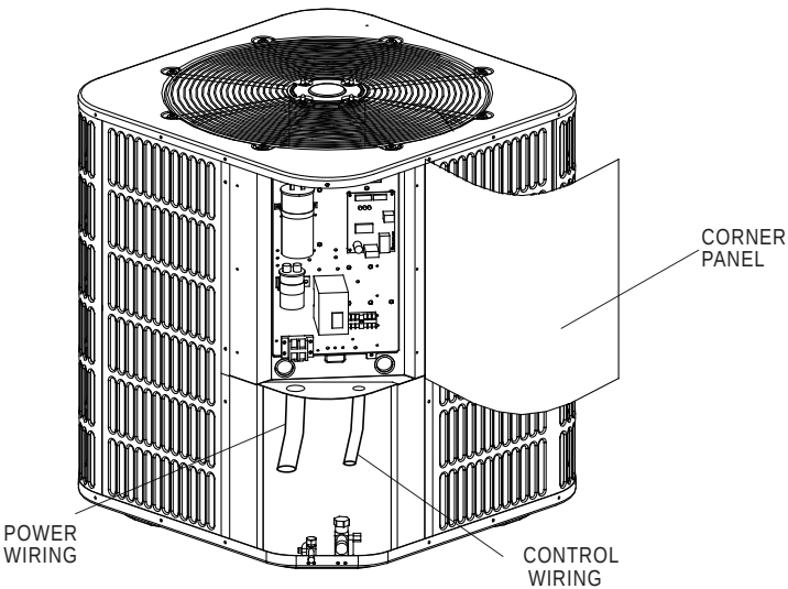
Typical Field Wiring
