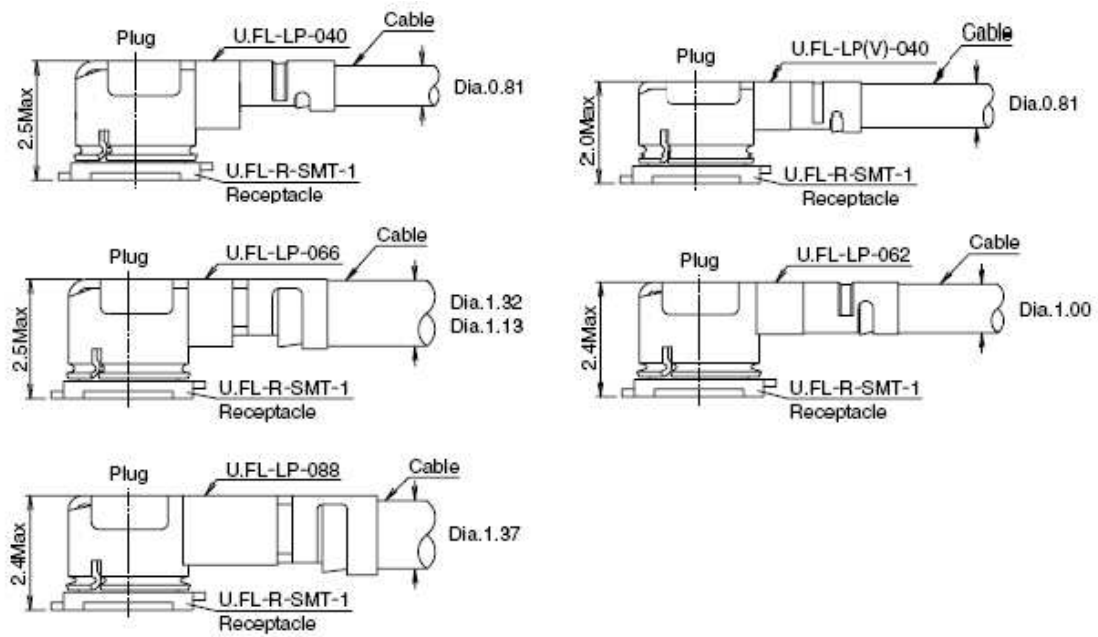
Figure 14: Space Factor of Mated Connectors (Unit: mm)
