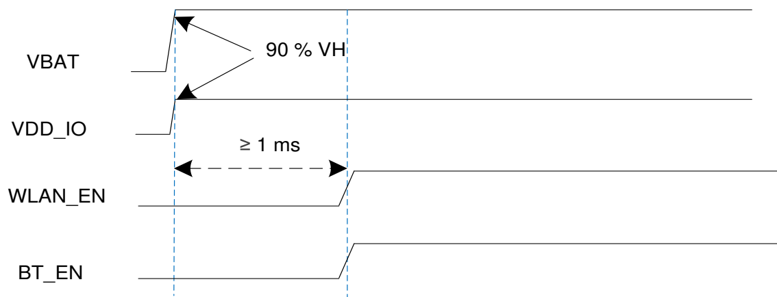
Figure 3: Power-up Timing
