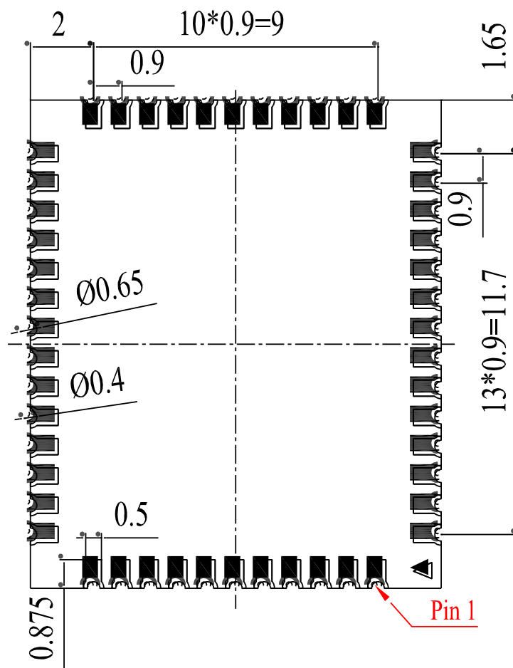
Figure 17: Bottom Dimension (Bottom View)
