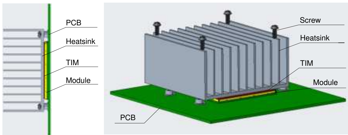
Figure 15: Placement and Fixing of the Heatsink
