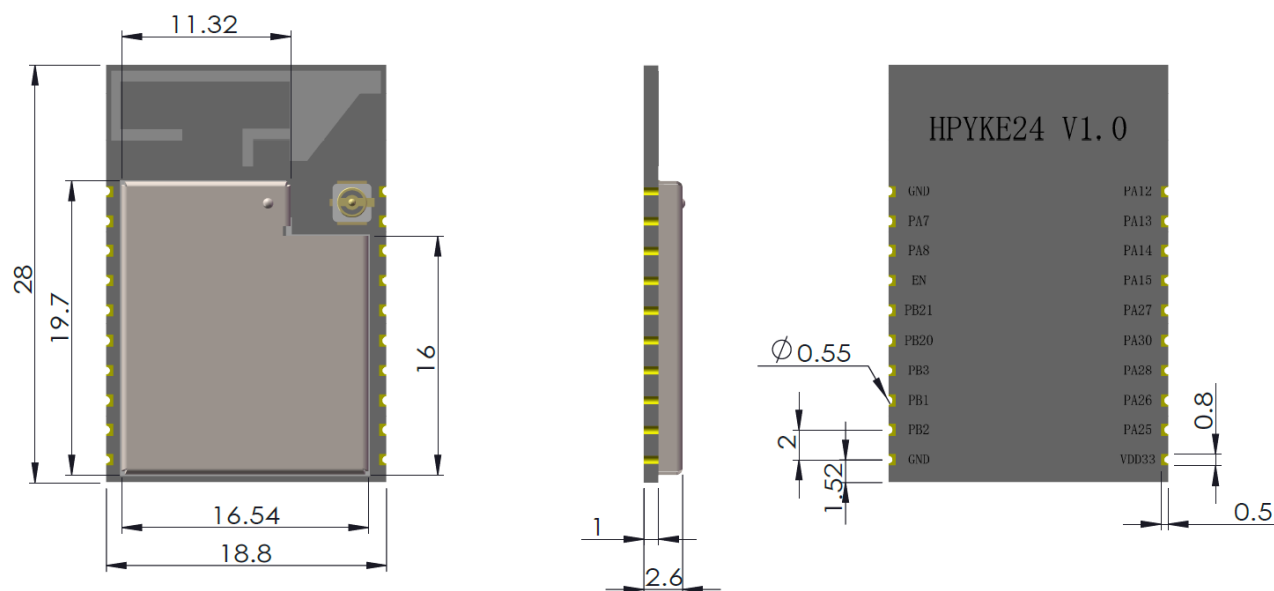
Figure 2. Module Dimension
