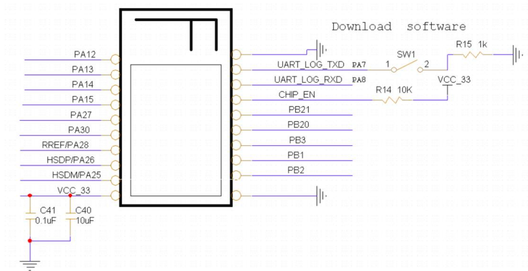
Figure 4. Reference schematic
