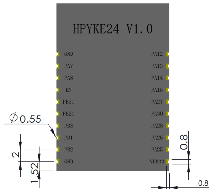
Figure 5. Module package
