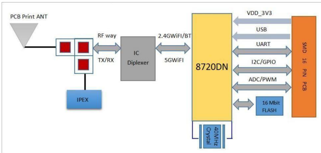
Figure 1. System architecture
