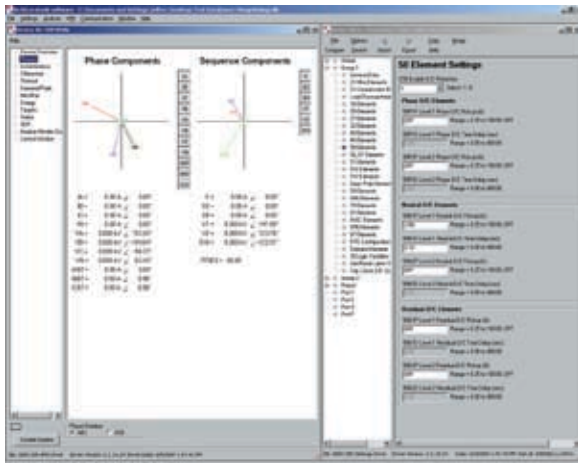
acSELEATOR QuickSet HMI simplifies configuration and troubleshooting.
