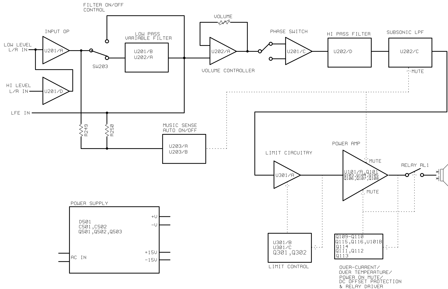
BLOCK DIAGRAM
