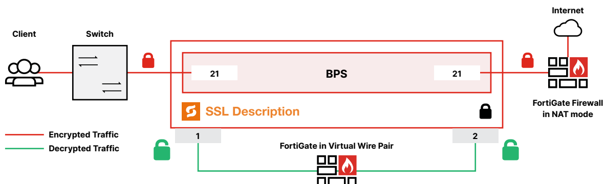
Figure 2-1: Gigamon Inline Solution with FortiGate NGFW.
