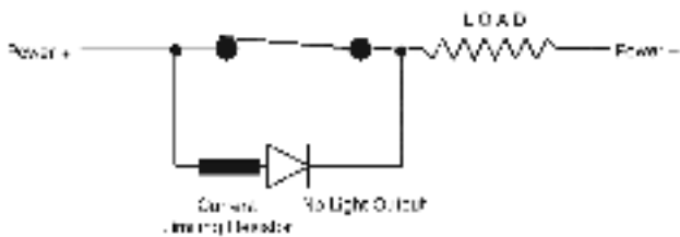
Figure 17. Wiring Diagram 2
