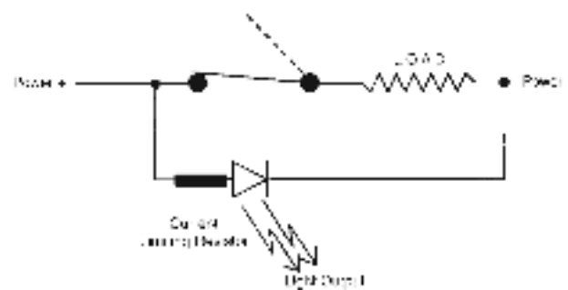
Figure 18. Wiring Diagram 3
