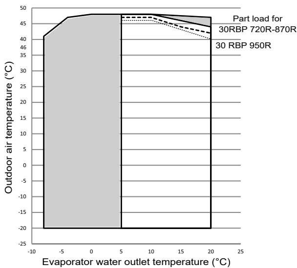
Operating range in cooling mode
