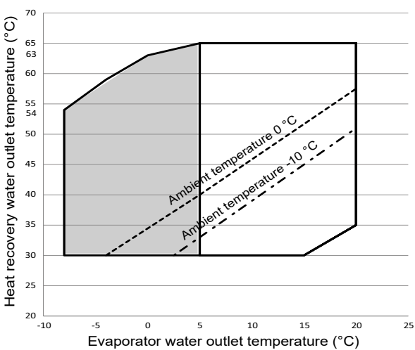
Operating range in heat recovery mode
