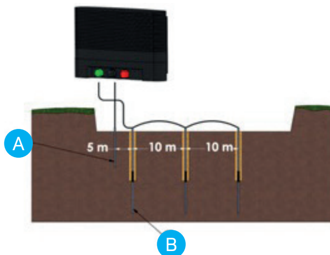
Figure 3.2: Earthing diagram for the MBS3000i model
