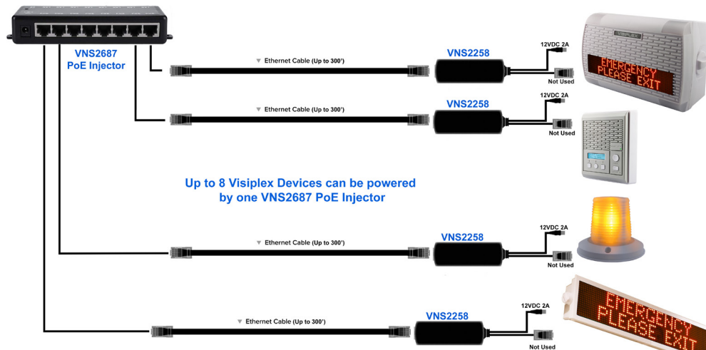
Low-Voltage Power Injector Wiring Diagram
