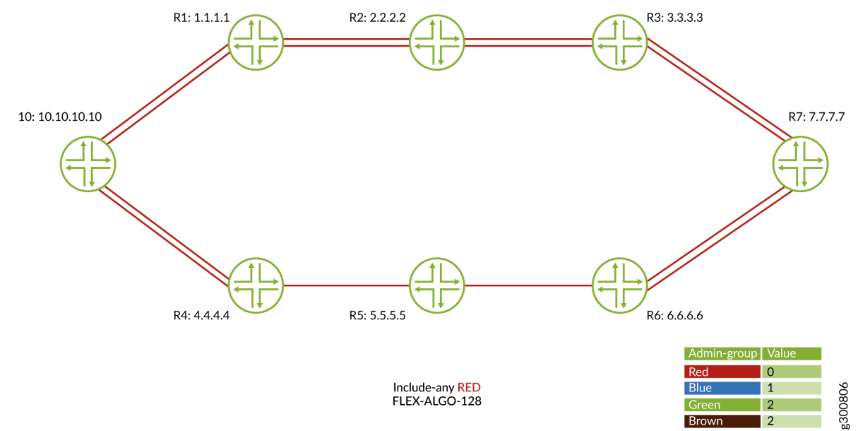
Figure 26: Traffic Flow for Flexible Algorithm Definition 128
