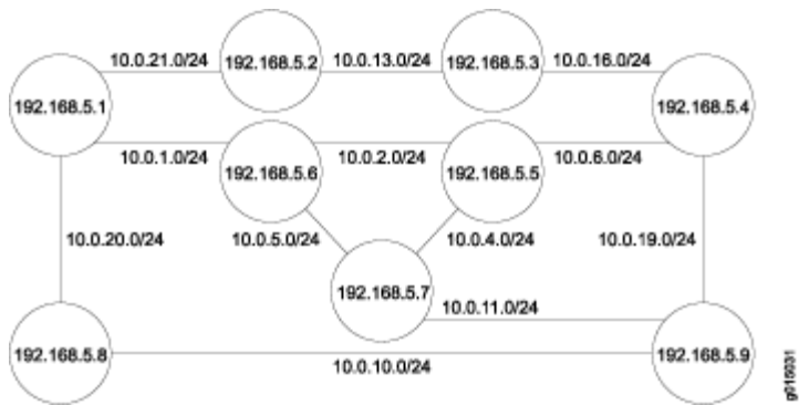
Figure 41: Sample OSPF Network Topology
