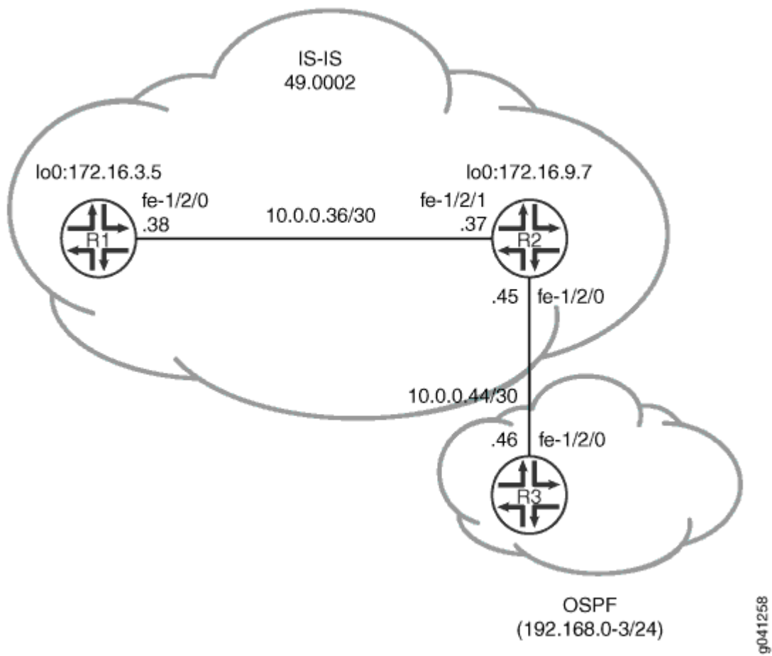
Figure 35: IS-IS Route Redistribution Topology
