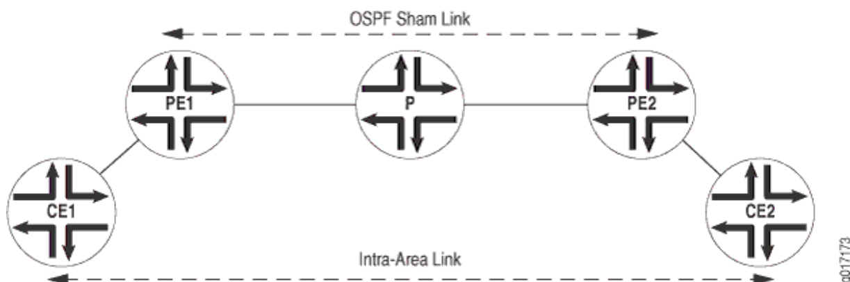
Figure 36: OSPFv2 Sham Link
