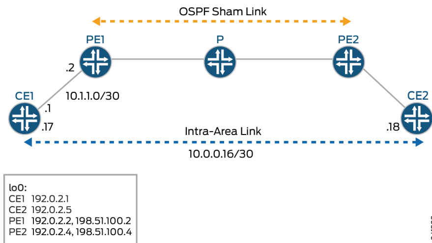
Figure 37: OSPFv2 Sham Link Example
