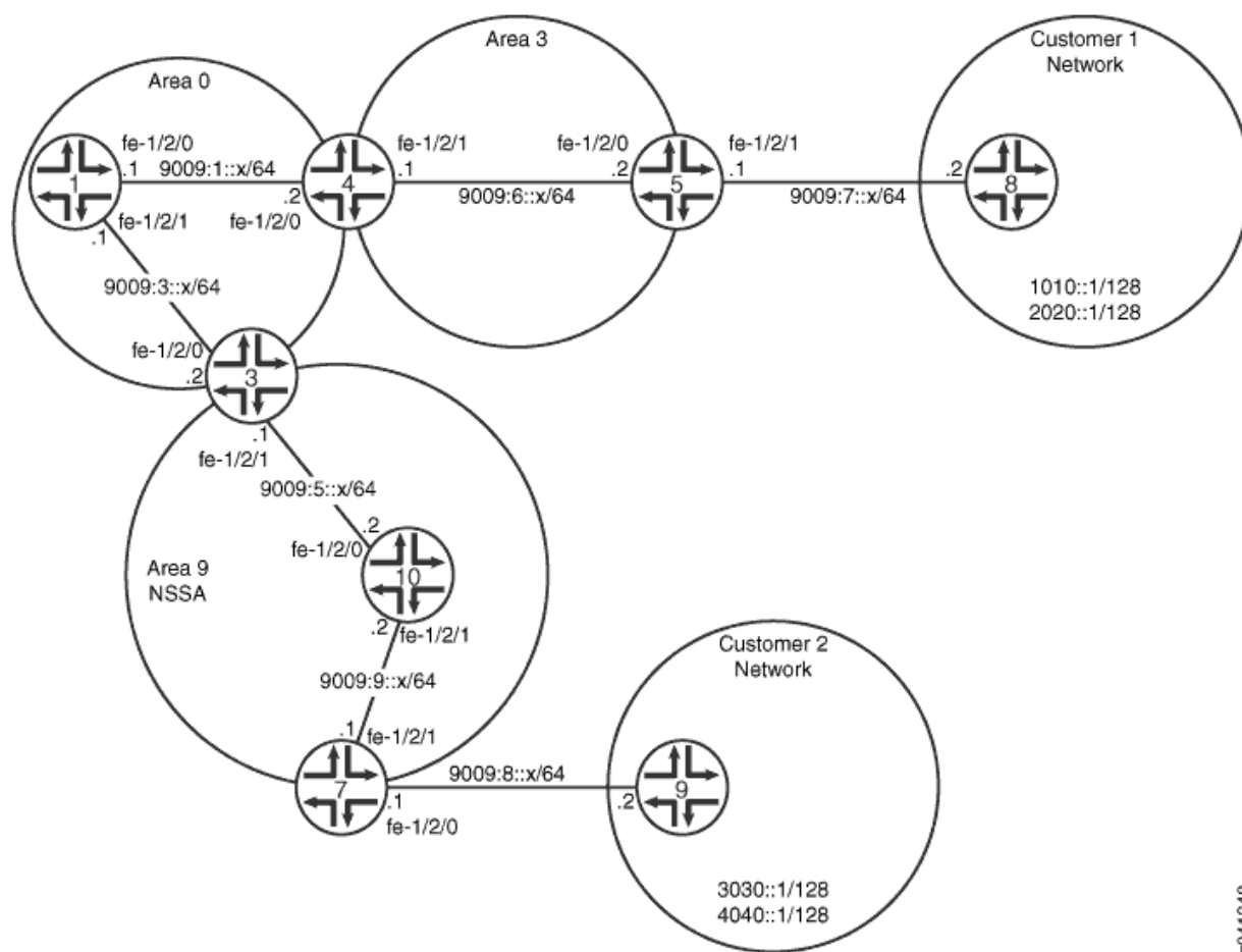
Figure 13: OSPFv3 Network Topology with an NSSA
