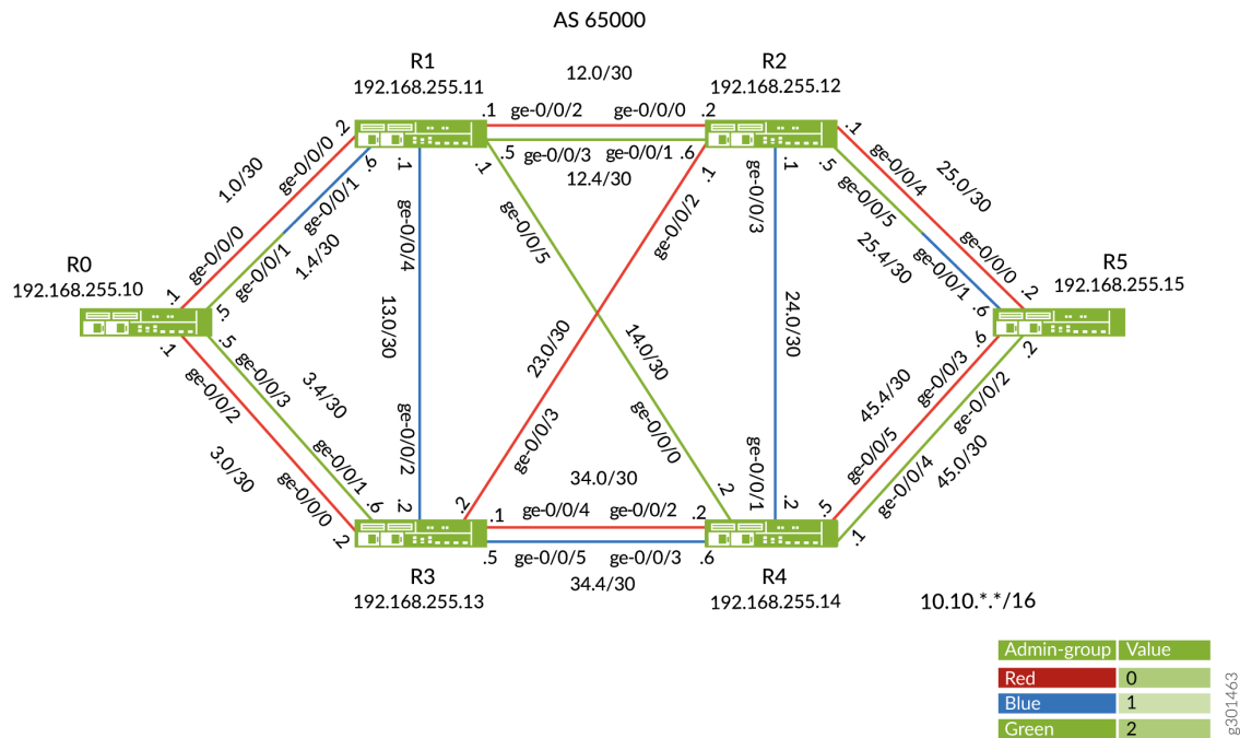
Figure 30: Flexible Algorithm Topology
