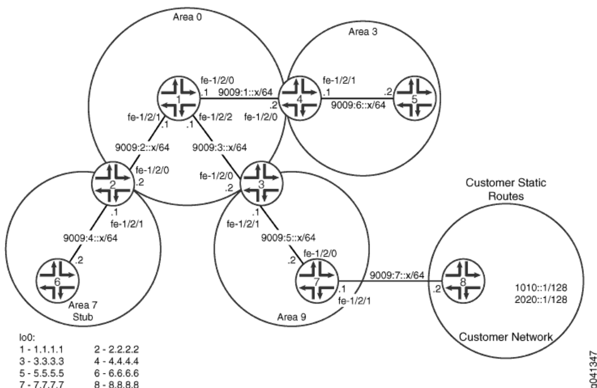
Figure 12: OSPFv3 Network Topology with Stub Areas
