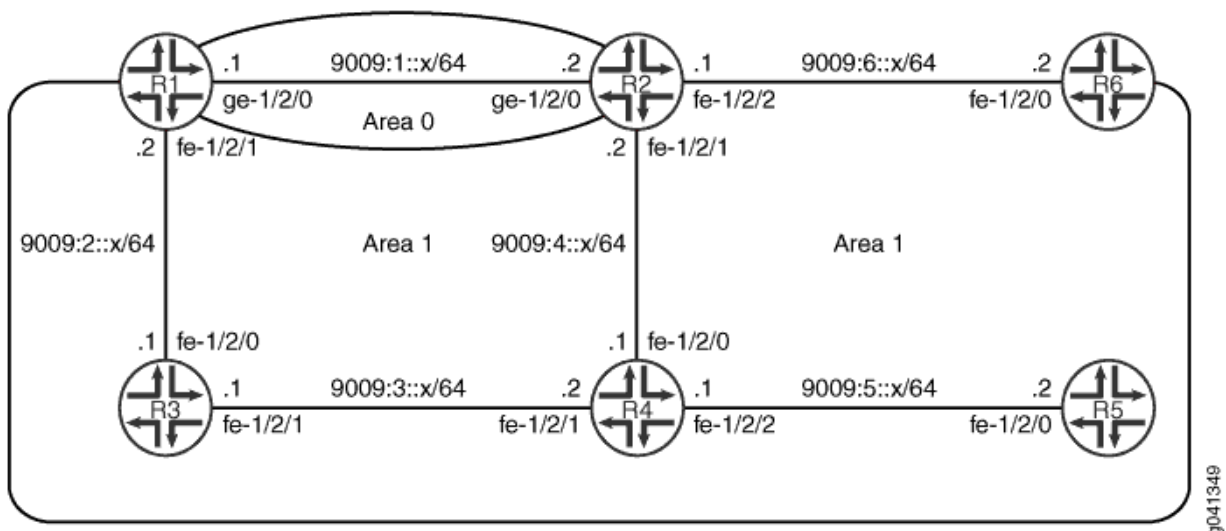
Figure 8: OSPFv3 Multiarea Adjacency
