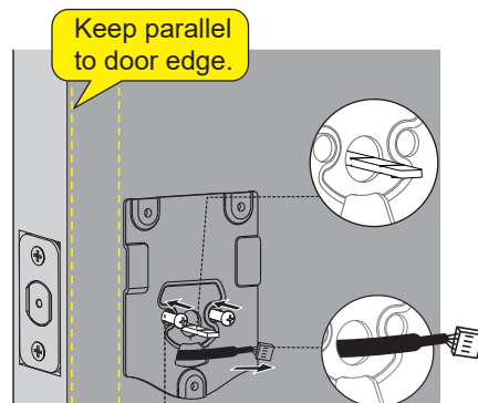
Mounting Plate Screws (J)
